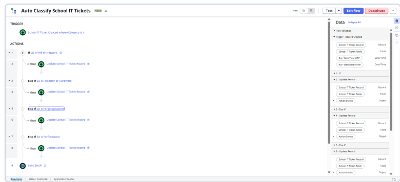
Figure 1: Flow Designer implementation of automatic classification requirement (FR-2).
